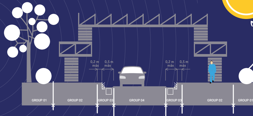
Location of groups acc. to their location on the public roads as per UNE-EN124-02:2015 definition.
